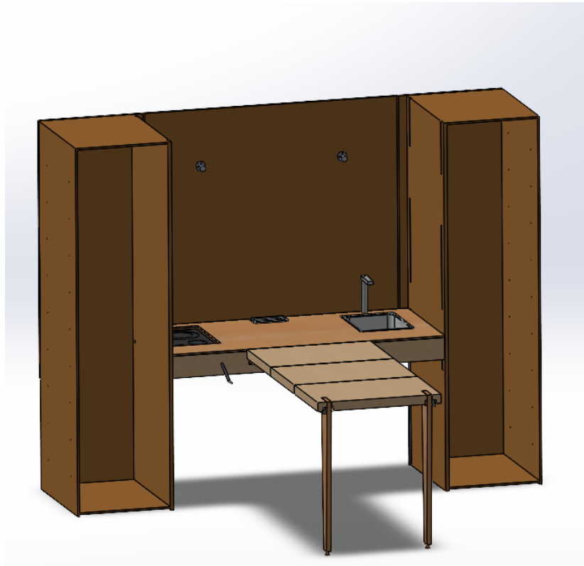
Fig.4: Merged prototypes
