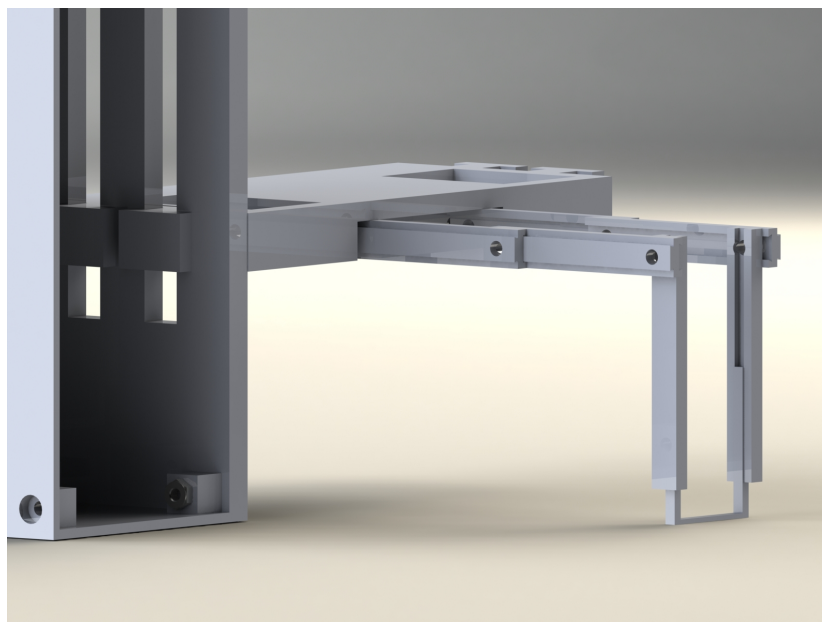
Fig.11: 3D model 2
